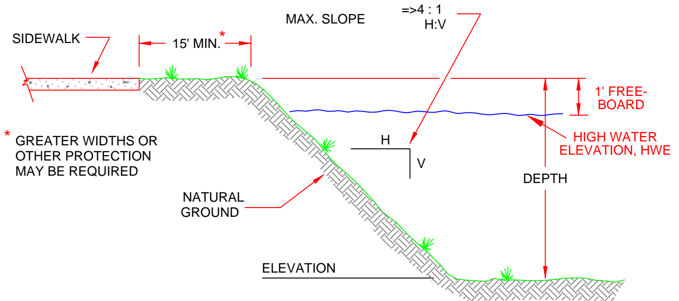
TYPICAL SECTION
